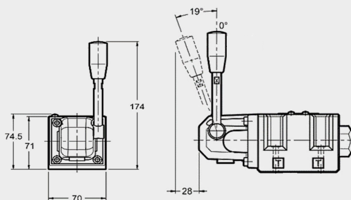
4/2-way
