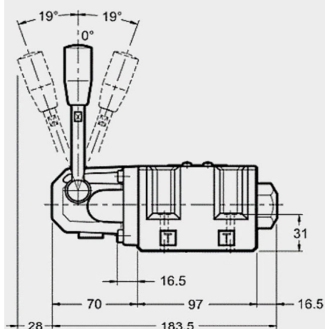
4/3-way
